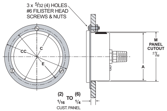
Front Flange (XFF)
