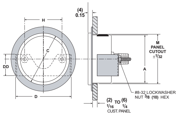
Retrofit Front Flange (XRF)
